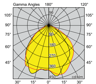
ORION LED PLUS 26W 6000K
