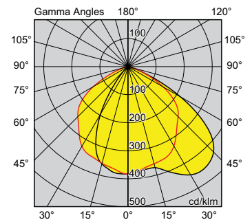
SOLARIS MCL 44W 4000K
