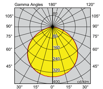
LUMEN SELECT 5000K 194W
