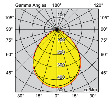
GENLED ONE 1200X300 45W 4000K
